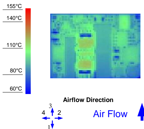
Figure 8. Thermal Image for Airflow Direction 3 (29A output, 75°C ambient, 200 LFM, typical Vin, open frame, unit soldered onto a fixture board)
